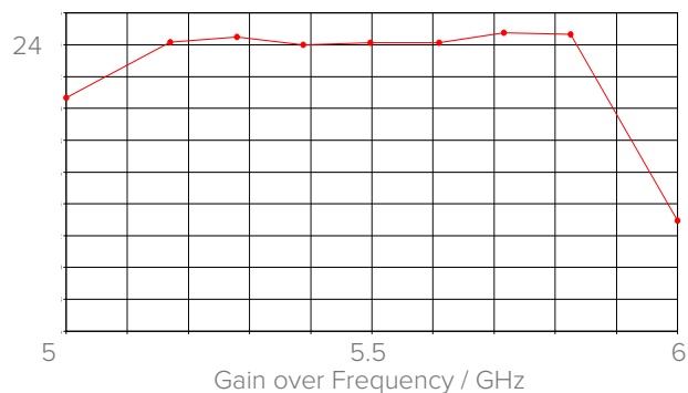
Vertical polarization
